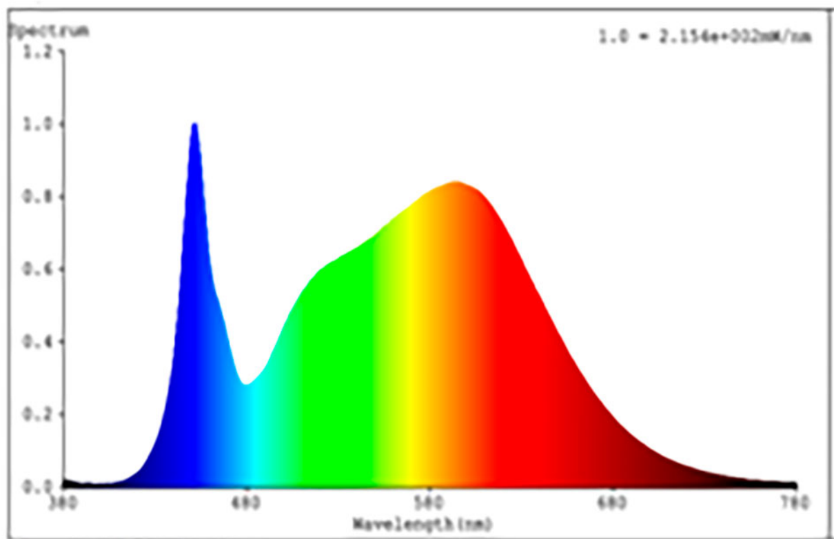
Spectral Distribution
